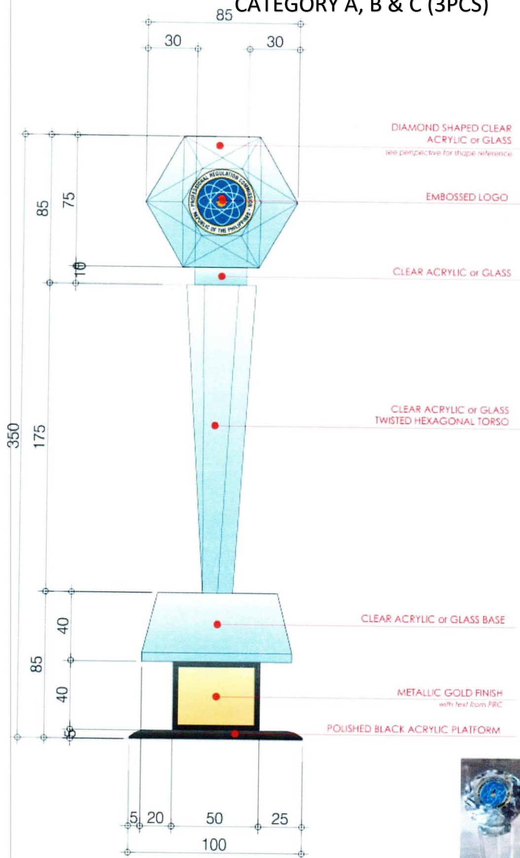
MOST OUTSTANDING IAPQA - LARGE FRONT ELEVATION SCALE 1:2MMS
